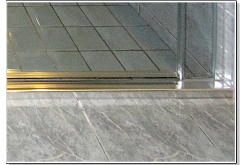
Bottom detail of a front-only screen, showing aluminium channel and polycarbonate strike along bottom of door, protecting against leakage
